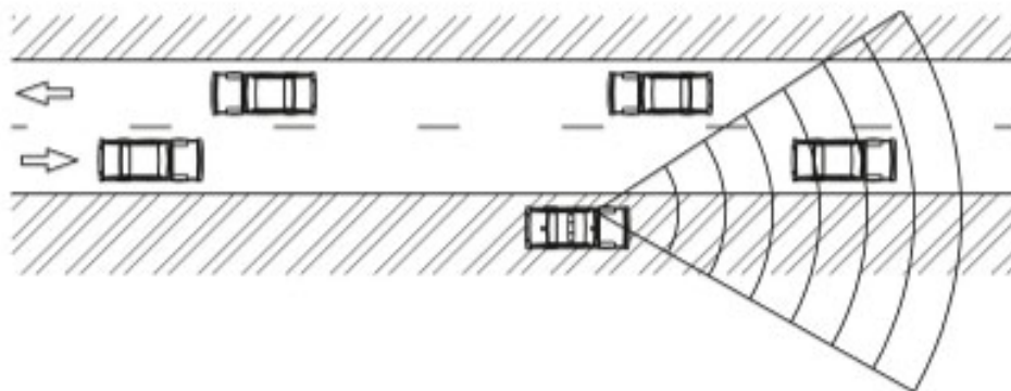
Figure 6.3 Tracking a target vehicle with a parked patrol vehicle and the radar in Stationary Mode.
